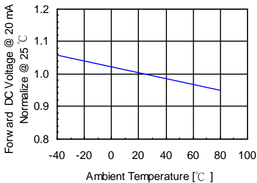
Fig 5. Forward DC Voltage vs. Temperature
